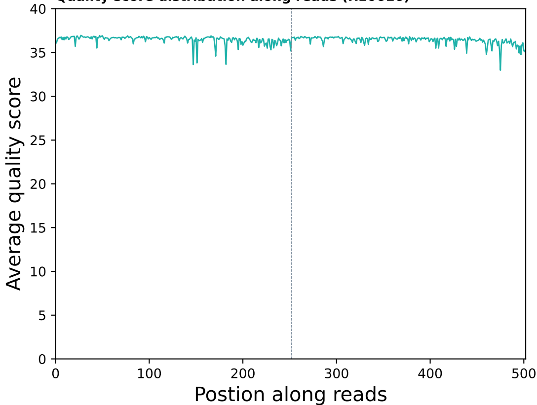
Quality score distribution along reads (R10616)
